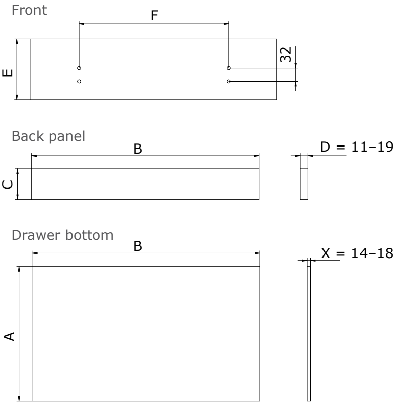
Cutting dimensions
