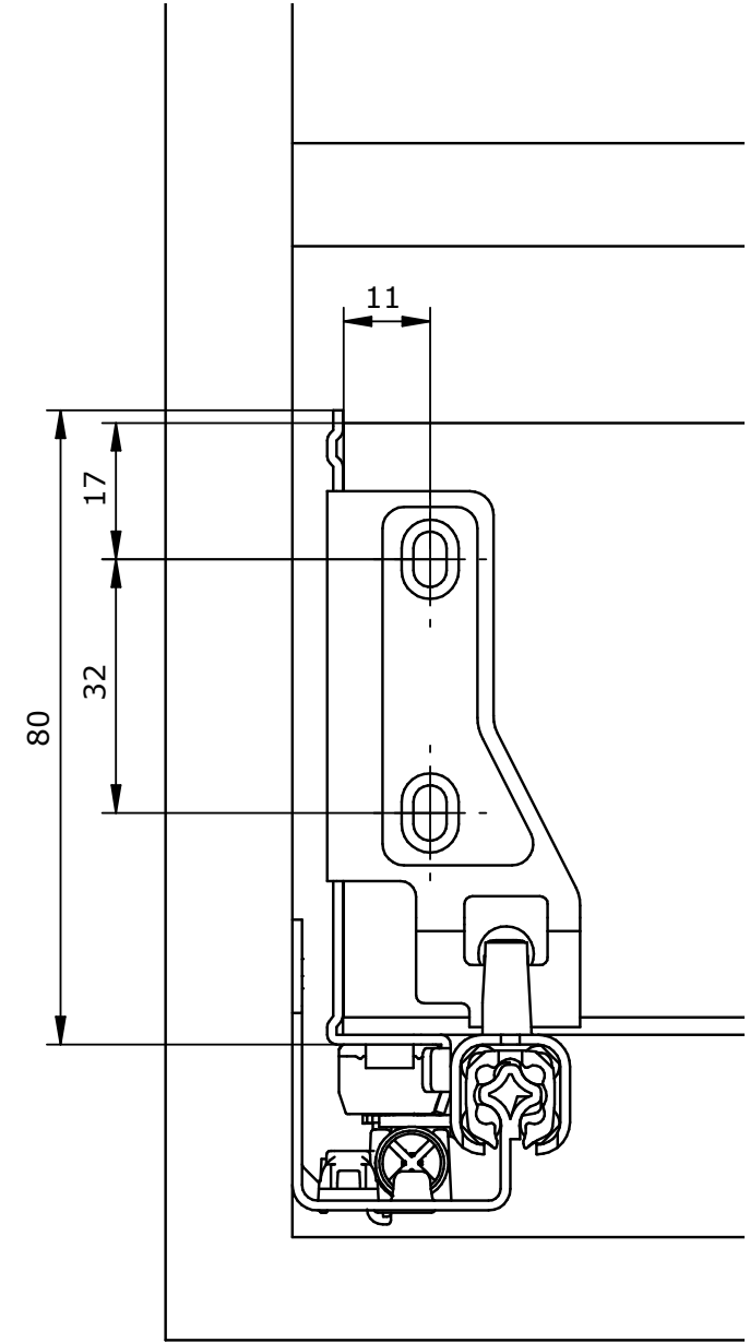
Installation dimensions back panel with Perfect
